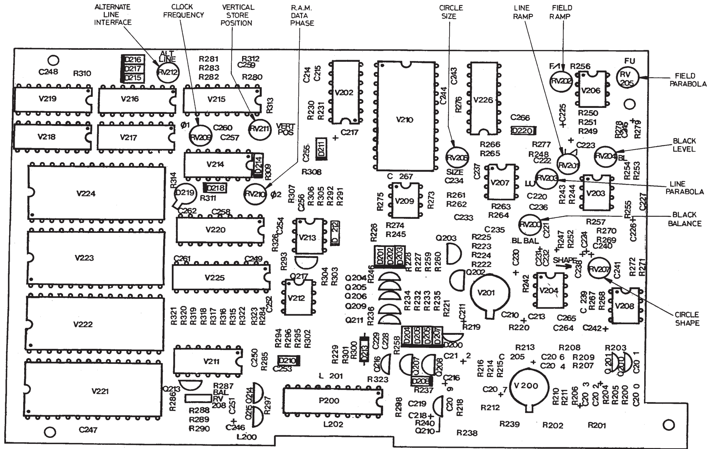
P4428 VIDEO PROCESSING BOARD ESA56493BA
