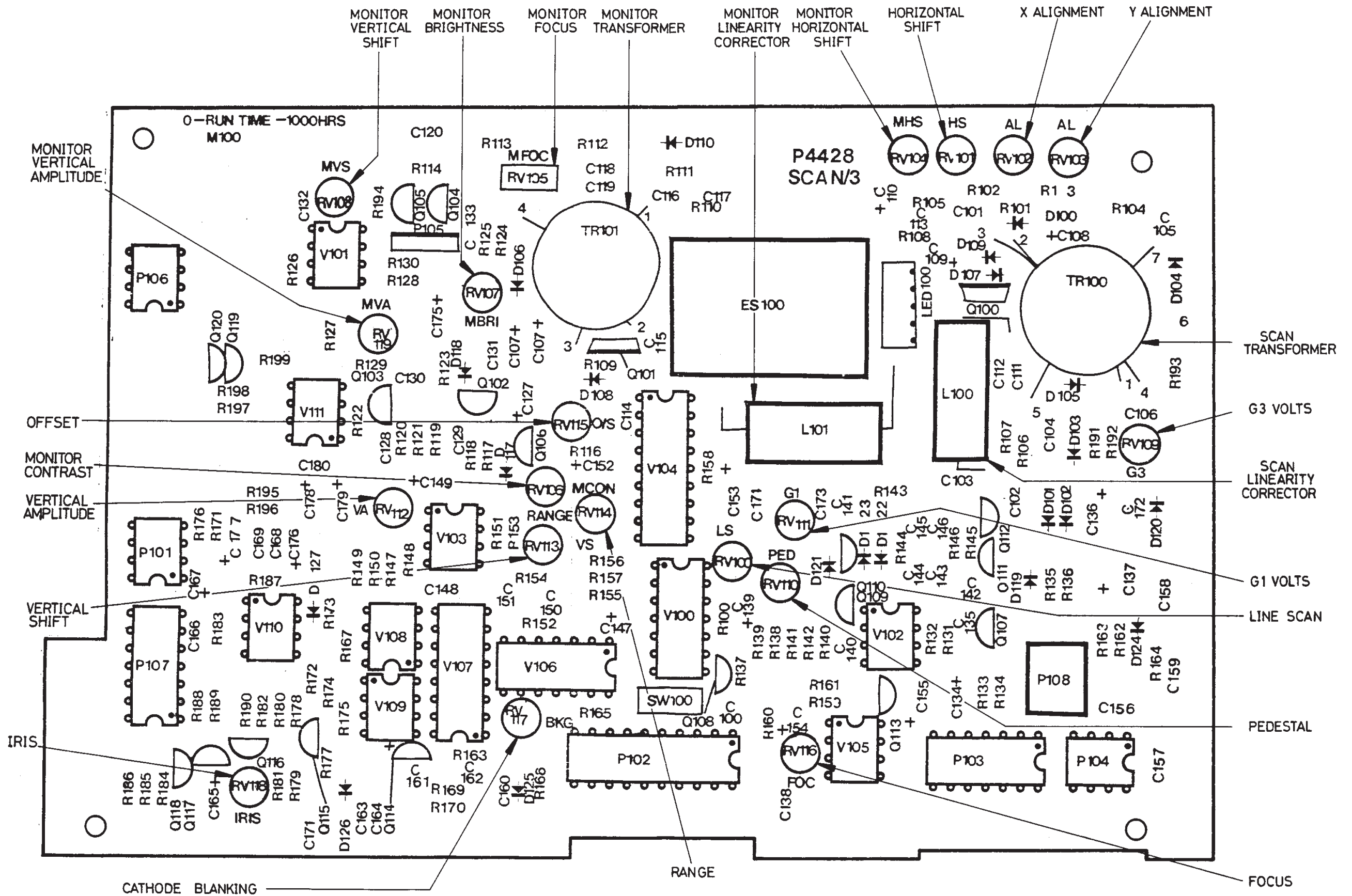
P4428 SCAN & MONITOR BOARD ESA56492AA
