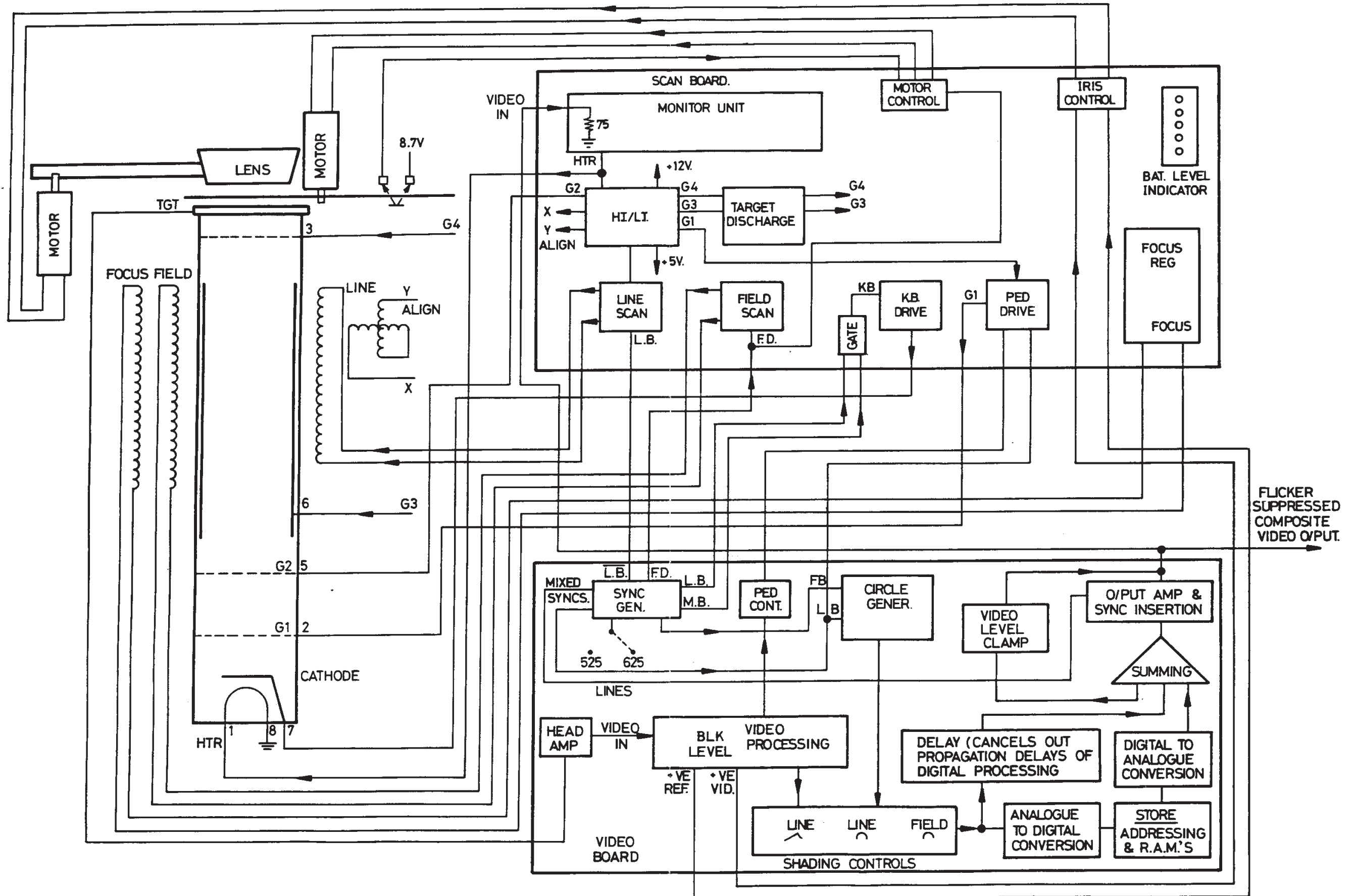
P4428 THERMAL BLOCK DIAGRAM
